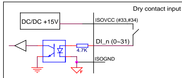
Figure 4-1 Dry contact inputs of EX-94164/AC
