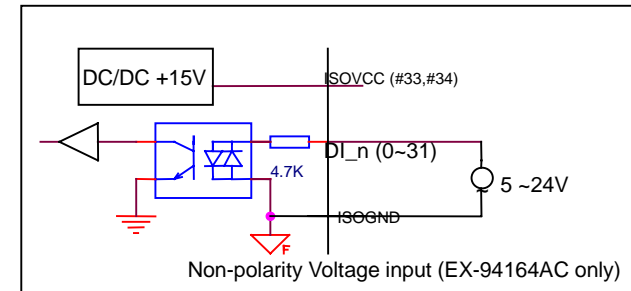
Figure 4-2 Voltage digital inputs of EX-94164/AC
