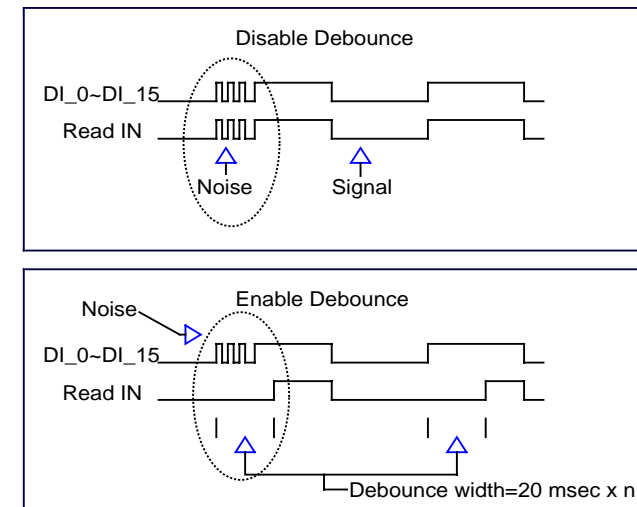
Figure 4-4 inputs debounce block diagram
