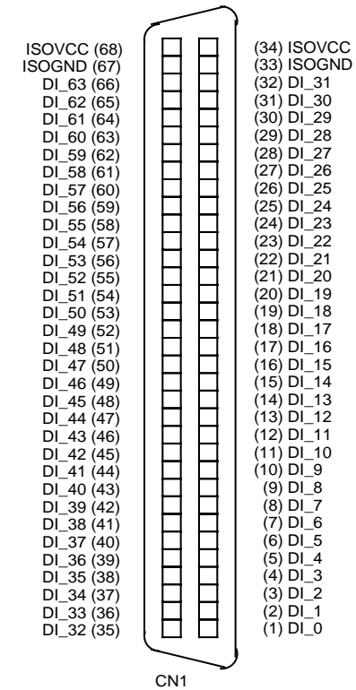
Figure 2.7 Pin Assignment of EX-94164/AC connector CN2
