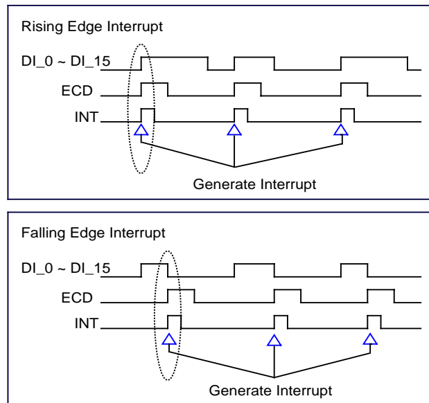
Figure 4-3 inputs interrupt block diagram
